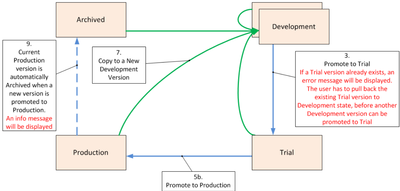
Figure 18 Creating a New DCA App Version
